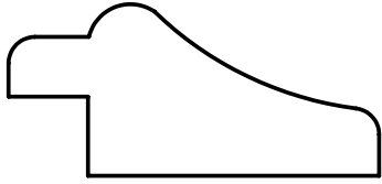
CM 701 13/16 X 1 3/4
